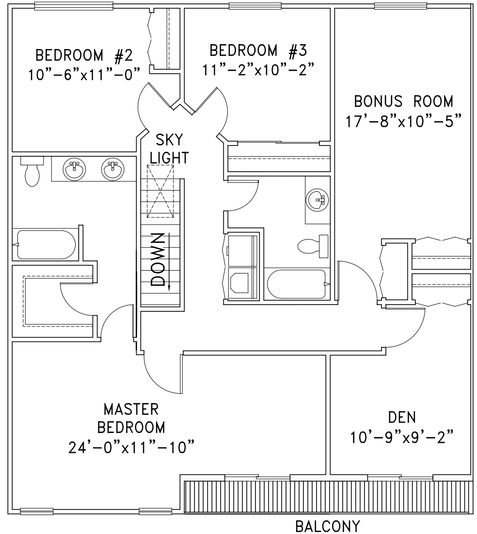
TOWNHOME W/ DOUBLE GARAGE LIVING AREA: 2218 S.F. GARAGE: 447 S.F.
